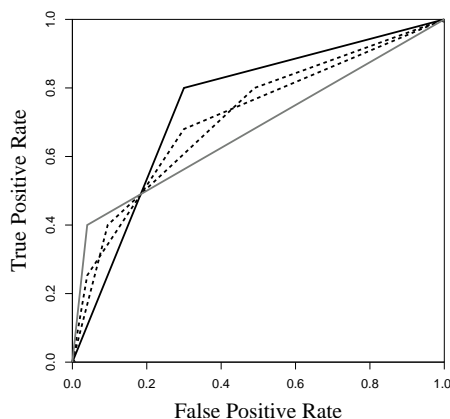
Figure 14. Vertical and Horizontal Averages of two ROC curves
