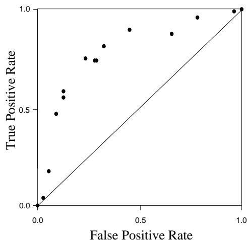
Figure 6. ROC Points for C4.5 on the Sonar dataset
