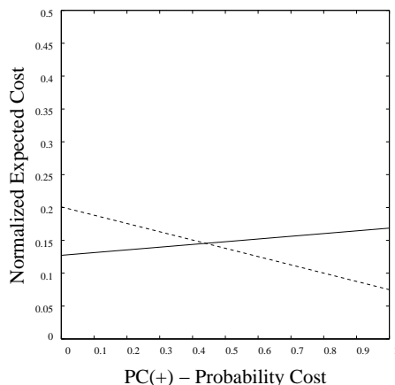
Figure 5. Japanese credit - Cost Lines for 1R (dashed line) and C4.5 (solid line)
